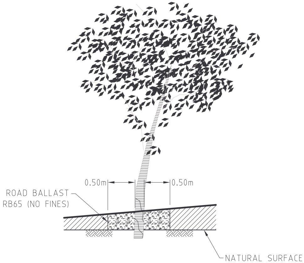
FILLING AT EXISTING TREE DETAIL NTS
