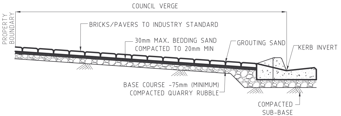
PAVED VEHICLE CROSSOVER SECTION
