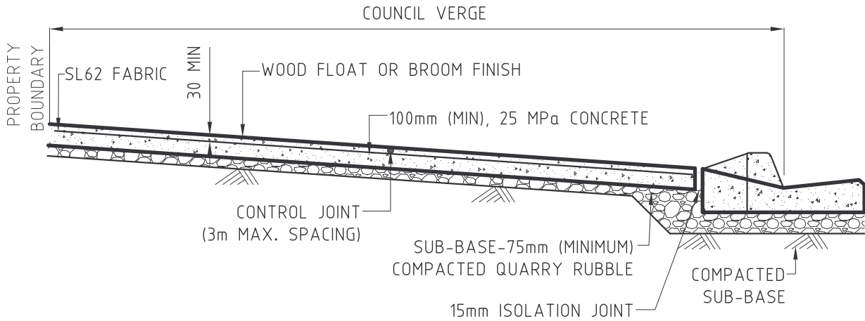
CONCRETE VEHICLE CROSSOVER SECTION
