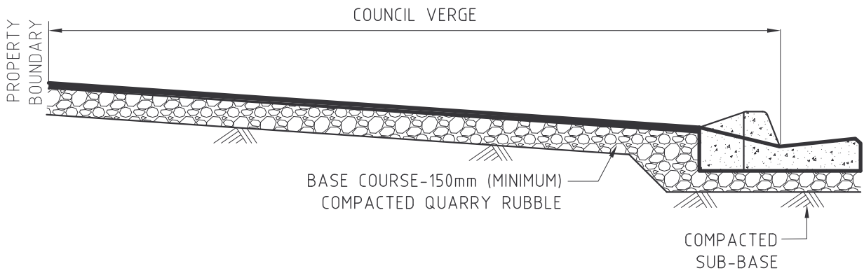
HOTMIX VEHICLE CROSSOVER SECTION
